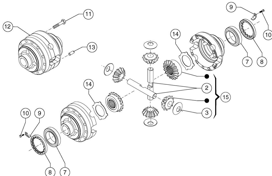
REAR AXLE - DIFFERENTIAL
